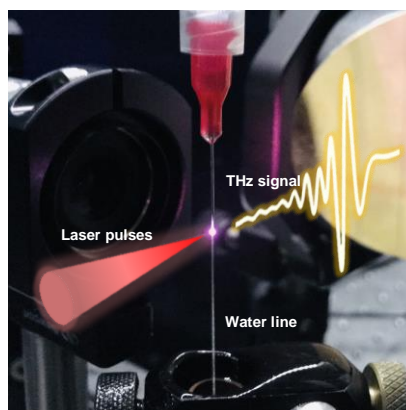
Figure: Laser induced micro-plasma in a water line, broadband THz wave emission is observed.
